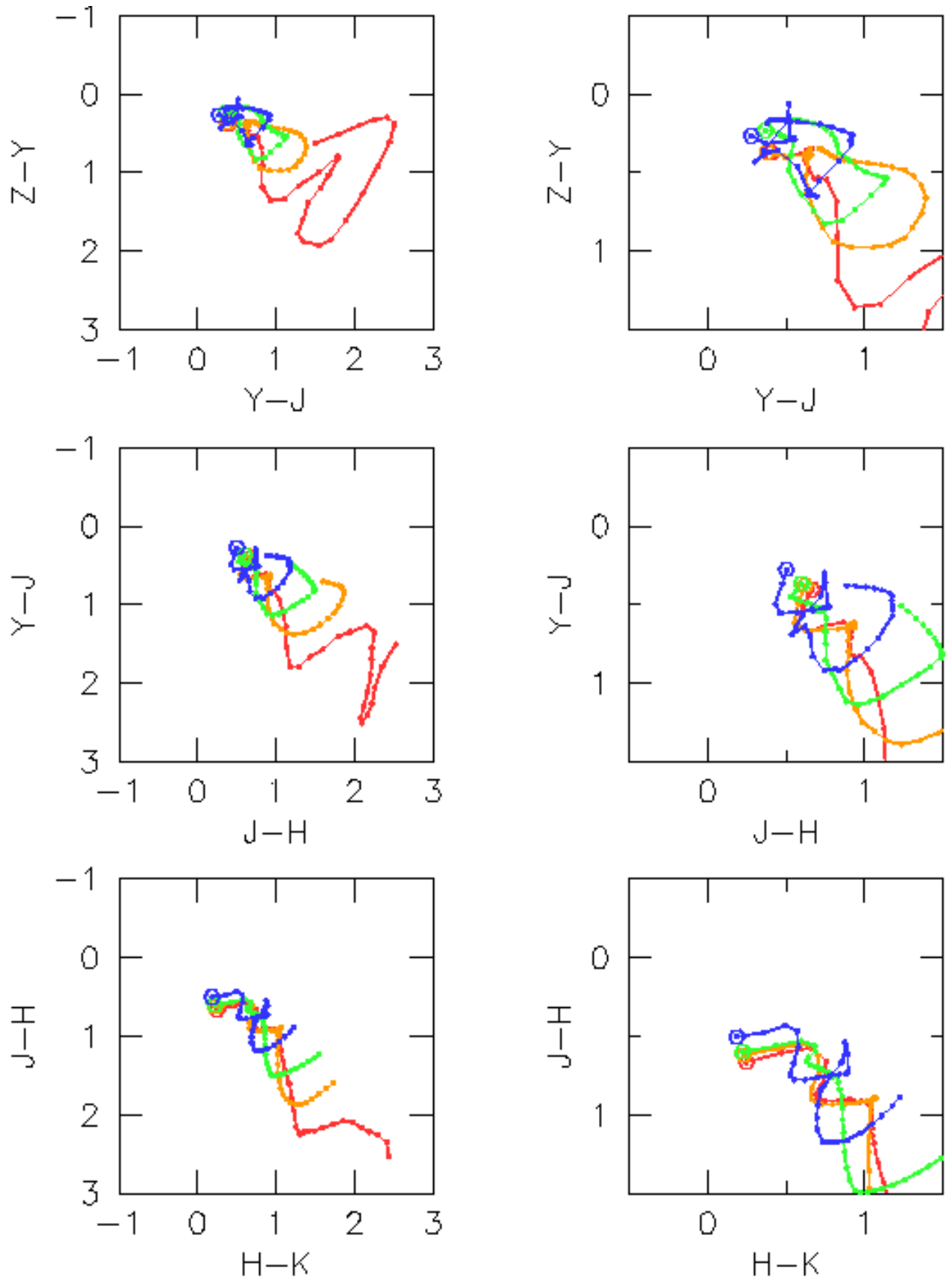
Figure 3. Top to bottom, three 2-colour diagrams of hypeprz galaxy templates, redshift range 0 < z < 3.6 , \Delta z = 0.1 , cycling through the colour sequence Z - Y , Y - J , J - H , H - K . Each right-hand panel is a 2\times expanded view of part of the corresponding left-hand panel. Key: E red, Sbc orange, Scd green, Im blue. For all curves z = 0 is marked by an open hexagon.
