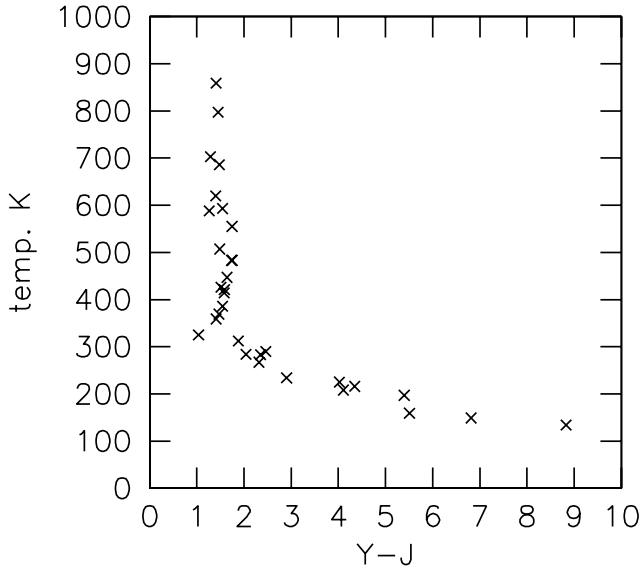
Figure 4. Temperature–colour relation of model cool brown dwarfs
