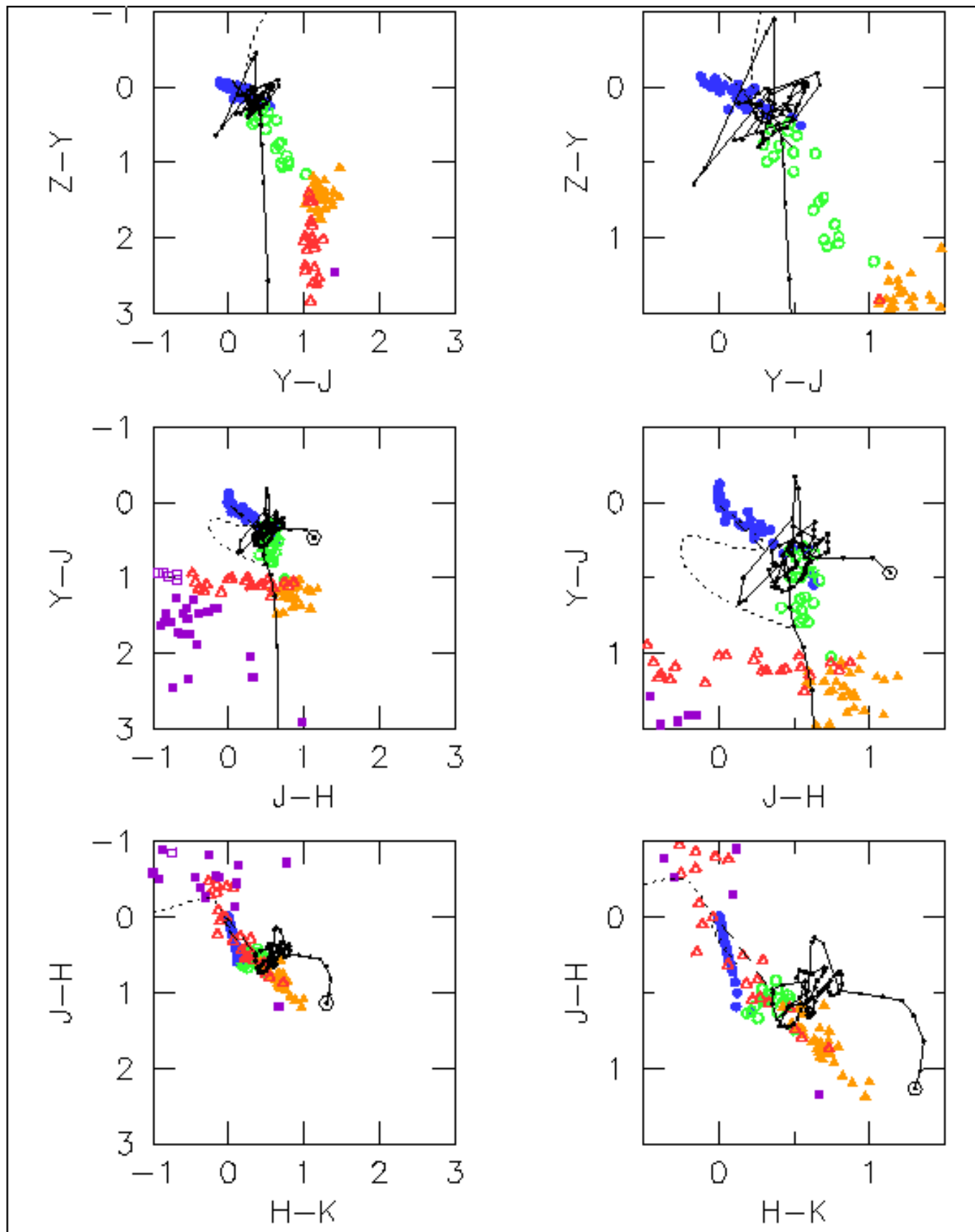
Figure 2. Top to bottom, three 2-colour diagrams of stellar sources, cycling through the colour sequence Z-Y , Y-J , J-H , H-K . Each right-hand panel is a 2\times expanded view of part of the corresponding left-hand panel. Key: BPGS O-K dwarfs blue \bullet ; M dwarfs green \circ ; L dwarfs orange \blacktriangle ; T dwarfs red \triangle ; Burrows model cool brown dwarfs purple \blacksquare ; Marley model cool brown dwarfs purple \square ; quasars 0 < z < 8.5 , \Delta z = 0.1 , solid black line, z = 0 marked by open hexagon; H white dwarfs dotted black line. He white dwarfs
