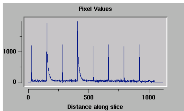
CDS dark frame, 8 channel readout, 1 sec exposure.
