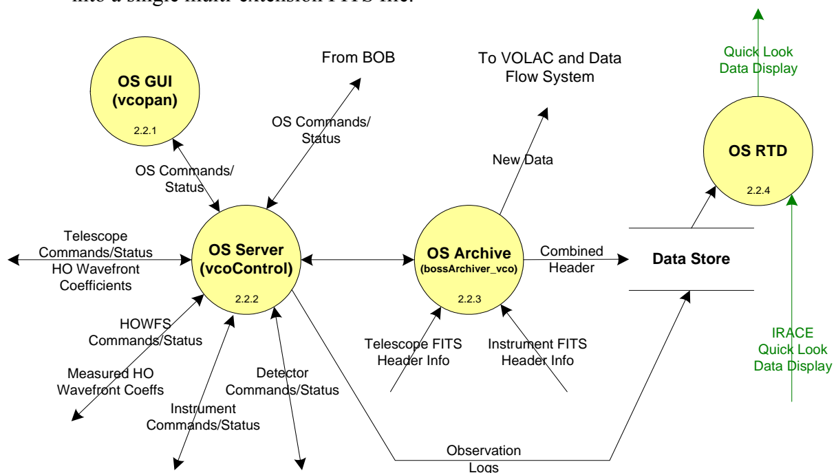
Figure 2 Decomposition of the VISTA IR Camera Observation Software
