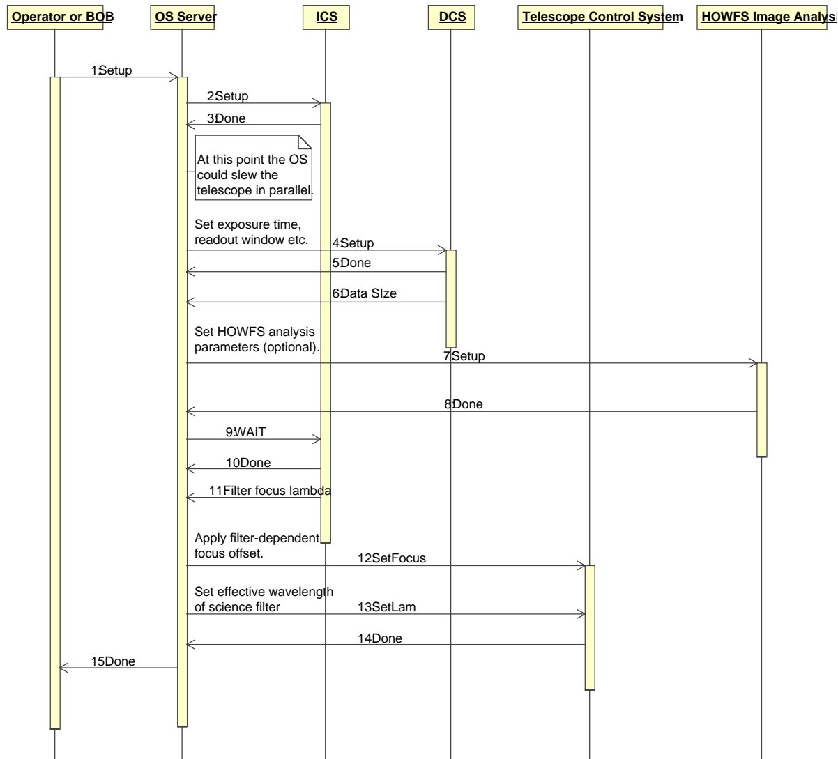
Figure 6 Sequence Diagram — Configure Instrument
