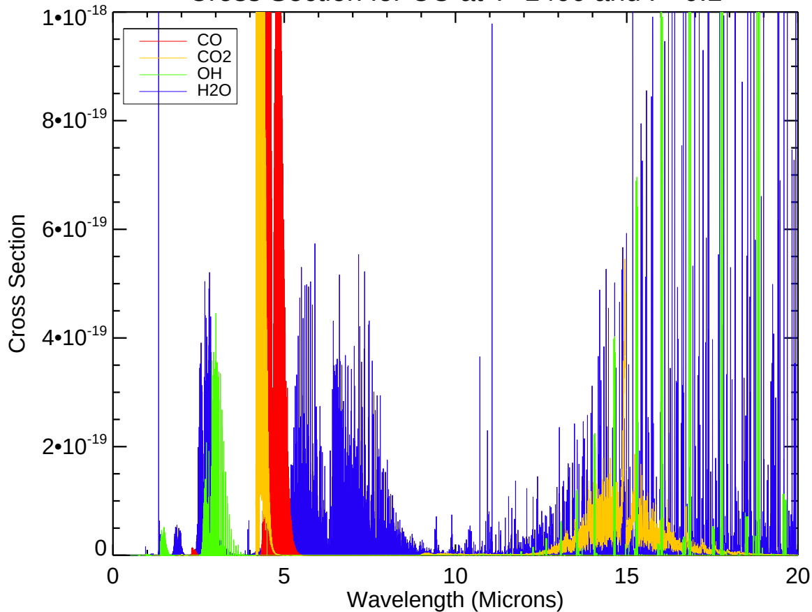
Cross Section for CO at T=1400 and P=0.1
